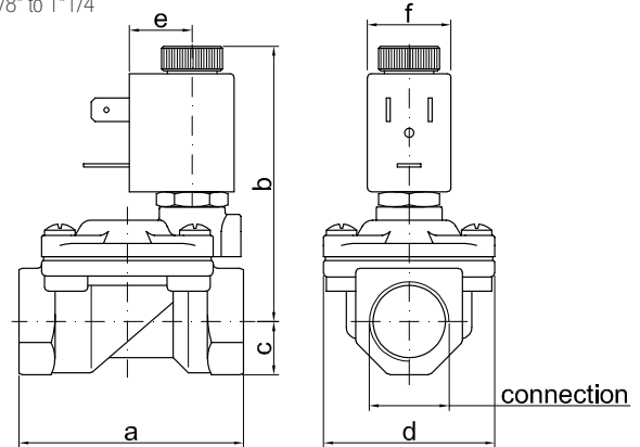
DN3/8" to 1"1/4
