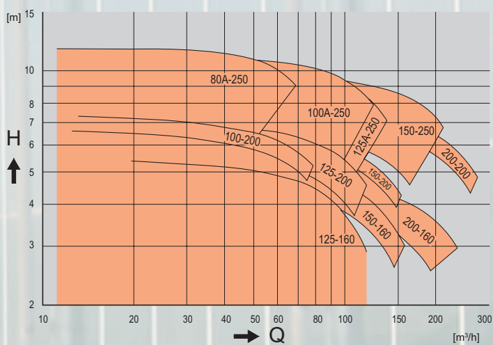
Hydraulic flow field CBH and CB at 50Hz 6 poles
