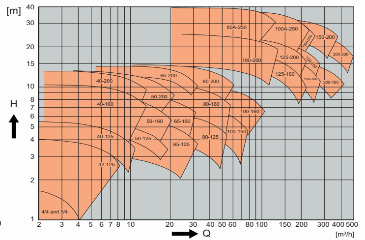
Hydraulic flow field CL and CLB at 60Hz 4 poles
