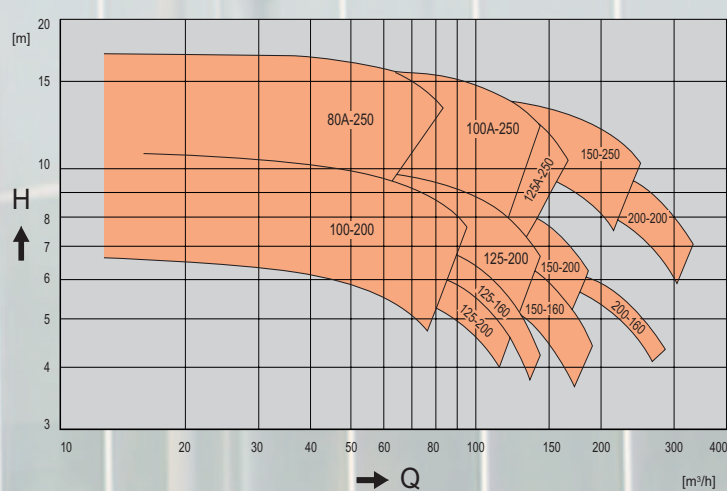
Hydraulic flow field CBH and CB at 60Hz 6 poles
