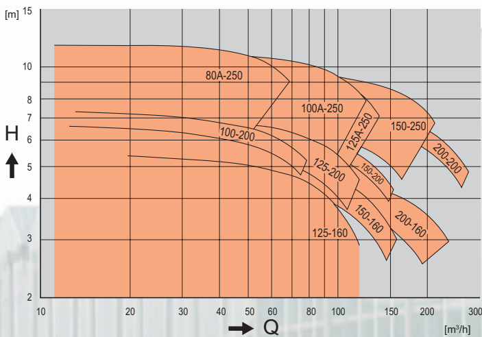
Hydraulic flow field CL and CLB at 50Hz 6 poles
