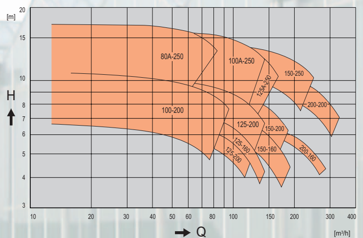
Hydraulic flow field CL and CLB at 60Hz 6 poles
