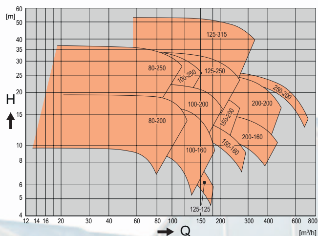
Hydraulic flow field CBH and CB at 60Hz 4 poles
