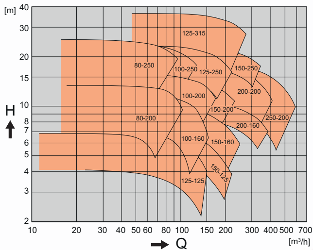
Hydraulic flow field CBH and CB at 50Hz 4 poles
