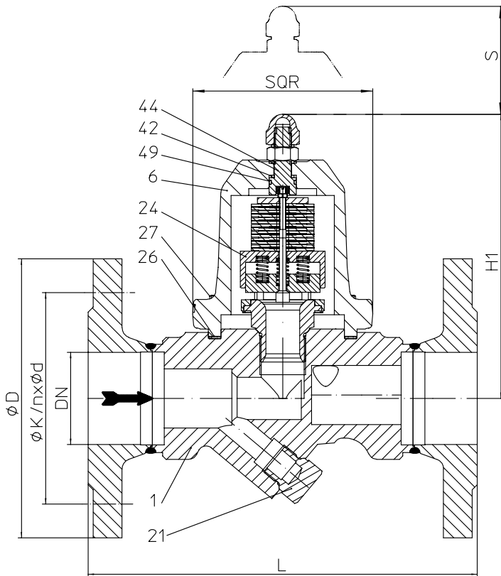
Fig. 650...1 with flanges
