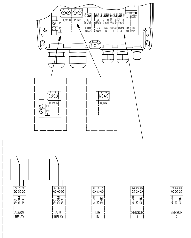
Fig. 29 Electrical connection of CU 300
