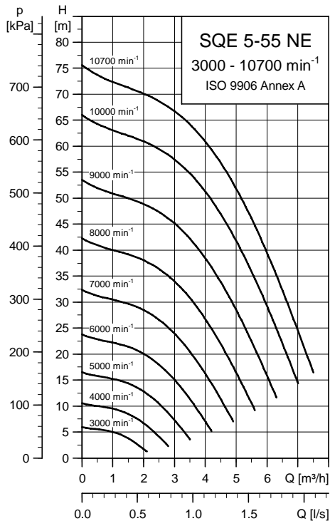
Fig. 25 Variable-speed curves
