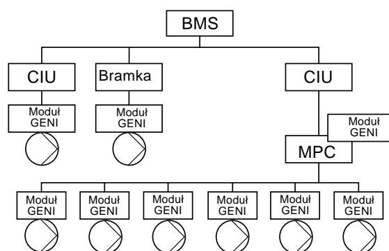
Rys. 16 MAGNA 25-40, 25-60, 25-80, 25-100, 32-40, 32-60, 32-80, 32-100, 40-60, 40-80, 40-100(D), 50-100 w systemie BMS
