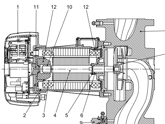
Rys. 20 UPE XX-120 FZ
