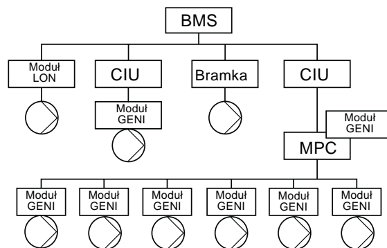
Rys. 17 MAGNA 32-120, 40-120, 50-60, 50-120, 65-60, 65-120 w systemie BMS
