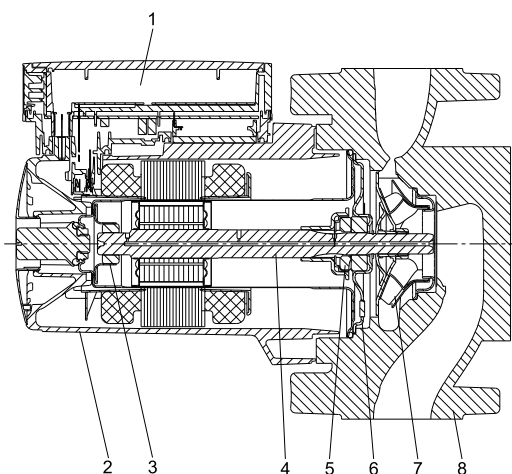
Rys. 19 MAGNA 32-120, 40-120, 50-60, 50-120, 65-60, 65-120
