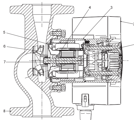
Rys. 18 MAGNA 25-40, 25-60, 25-80, 25-100, 32-40, 32-60, 32-80, 32-100, 40-60, 40-80, 40-100, 50-100
