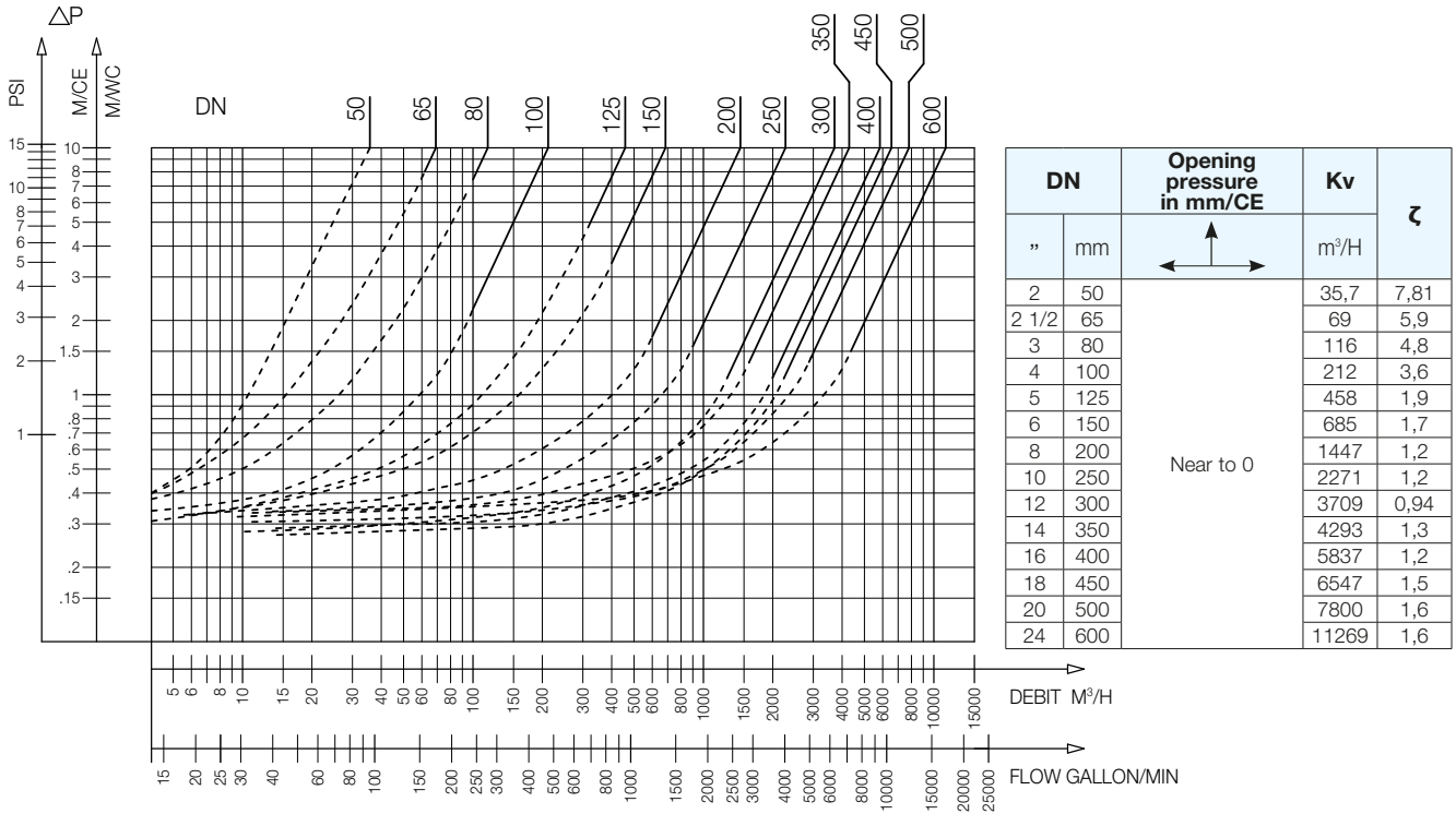
805 - Headloss chart
